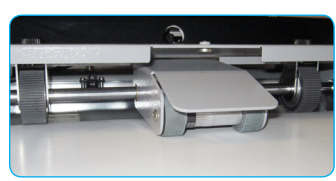
High-capacity feeder with three feed rollers plus two auxiliary feed wheels for consistent feeding
